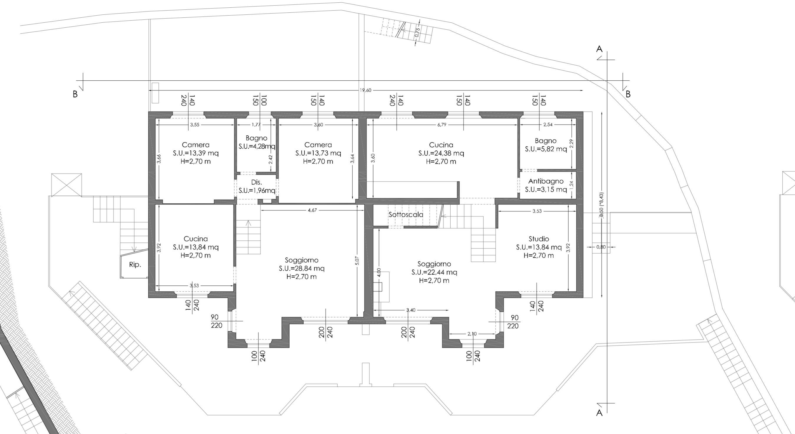
PIANO TERRA
