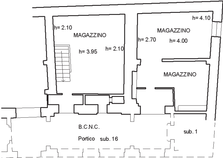
PIANO TERRA
